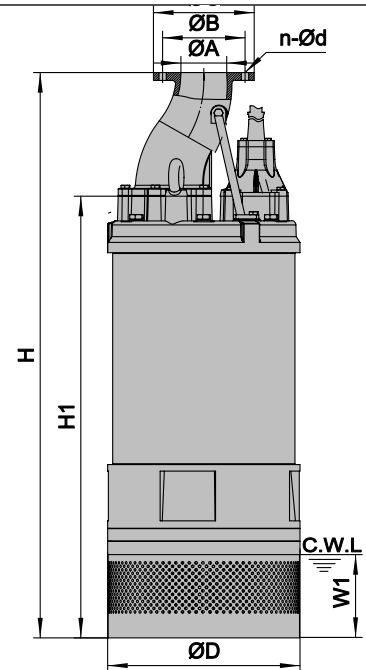
C.W.L:Continuous running water level
