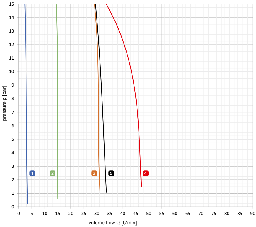
Performance chart VISCOPOWER at 3.000 mPas with PTFE stator
