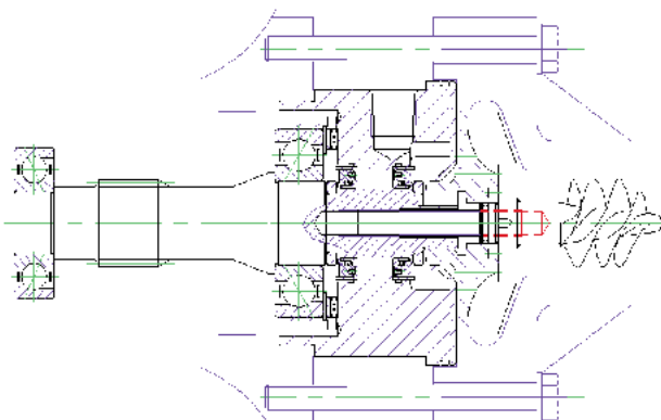
Single Seal Arrangement
